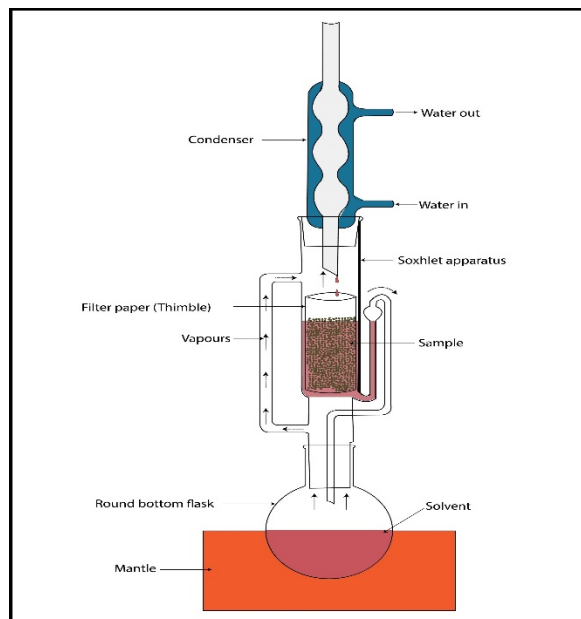
Fig. 1: Soxhlet apparatus for chemical extraction.
