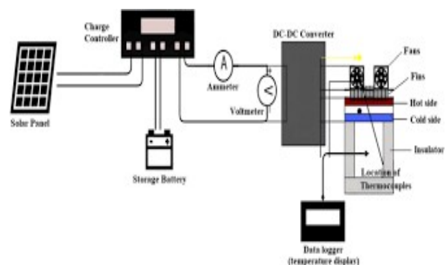
Fig.1 Block Diagram for Solar Powered Refrigeration
