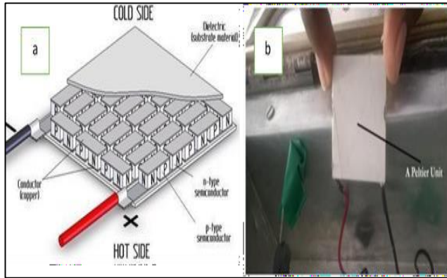
Fig.2 (a) Systematic Diagram of Peltier Effect (b) Peltier Module (TIC 12073)
