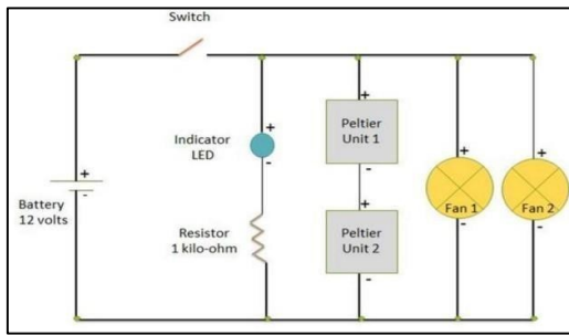
Fig.3 Circuit Diagram of the Experimental Study
